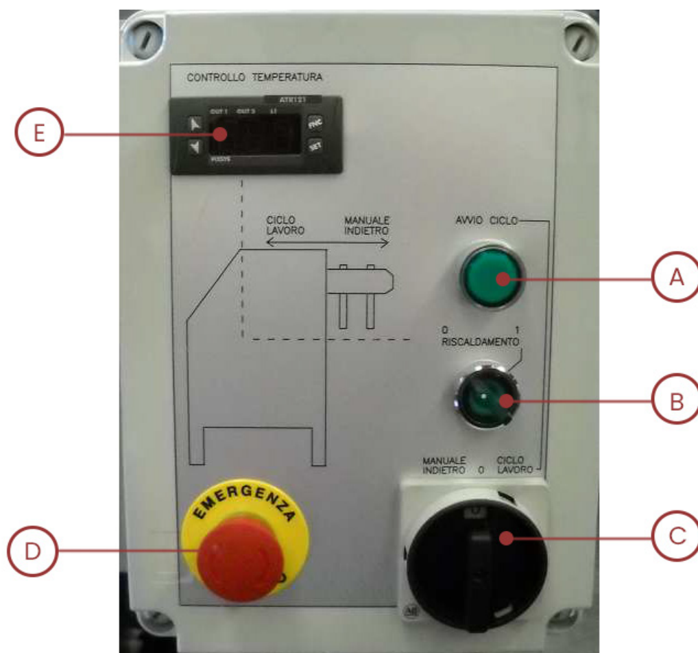
FIG. 1 Control panel
